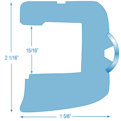
R1019 3/4" Hollow SS Trim
