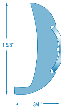
R1580 3/4" Hollow SS Trim
