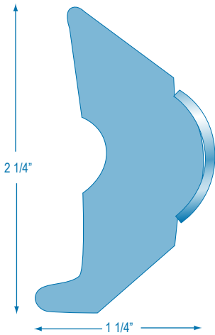
R1093 1" Hollow SS Trim
