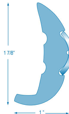
R1707 3/4" Hollow SS Trim
